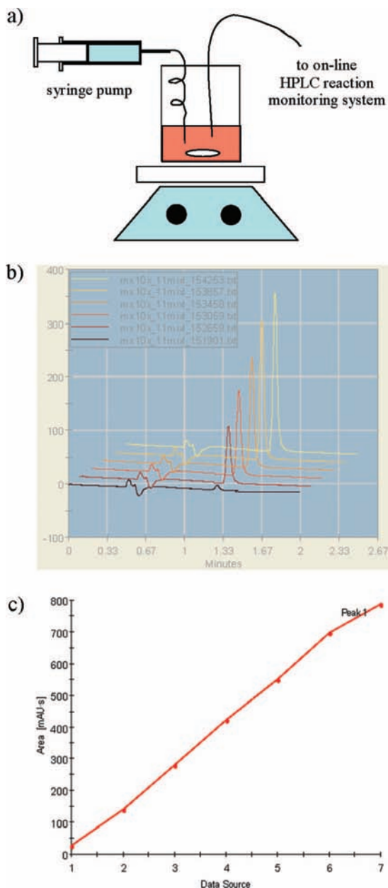
Figure 5. HPLC timecourse monitoring of the syringe pump addition of solution of propiophenone to acetonitrile/water. (a) Experimental setup; 2 mg/mL solution of propiophenone in 80% acetonitrile/water added via syringe pump (3 mL/h) to 5 mL of solution of 80% acetonitrile/water. (b) Waterfall plot showing stacked chromatograms with increasing peak area vs time. (c) Plot of integrated peak area vs time. HPLC and sampler conditions were those described in Figure 3, with additional conditions of a 0.8 min equilibration time, a 10 \times sample dilution setting using 80% acetonitrile/water as diluent, and a sampling interval of 4 min.
