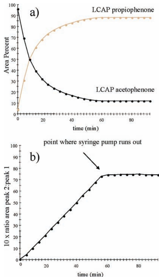
Figure 6. HPLC timecourse monitoring of the syringe pump addition of a solution of propiophenone to a solution of acetophenone in acetonitrile/water. The conditions were as follows: 1 mg/mL solution of propiophenone in 80% acetonitrile/water added to 1 mL of 0.3 mg/mL acetophenone in 80% acetonitrile/water at a rate of 5 mL/h; HPLC method as in Figure 5. (a) Plot of LCAP vs time. (b) Plot of the function of the ratio of the two peak areas vs time, revealing the point at which syringe pump ran out of liquid.
